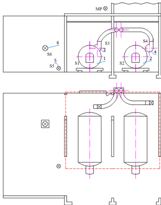
Fig.1. Layout of boiler room
