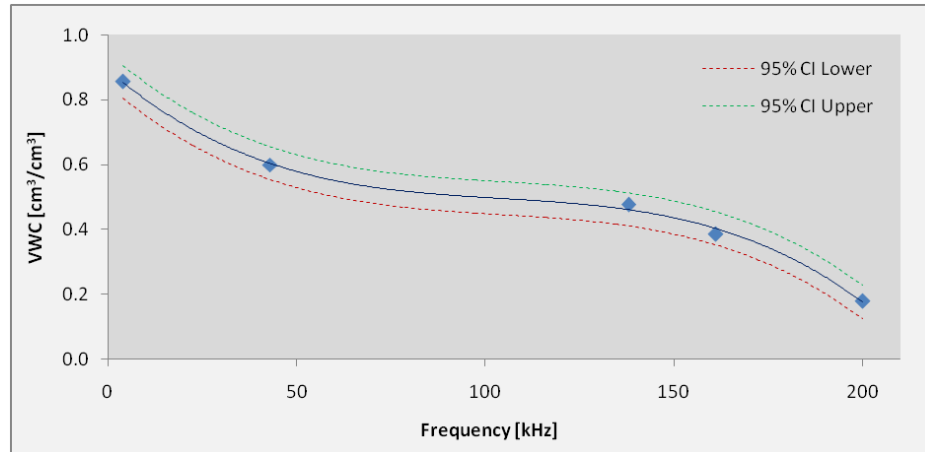
Figure 4. Sensor measurements and calibration curve in Compost soil
