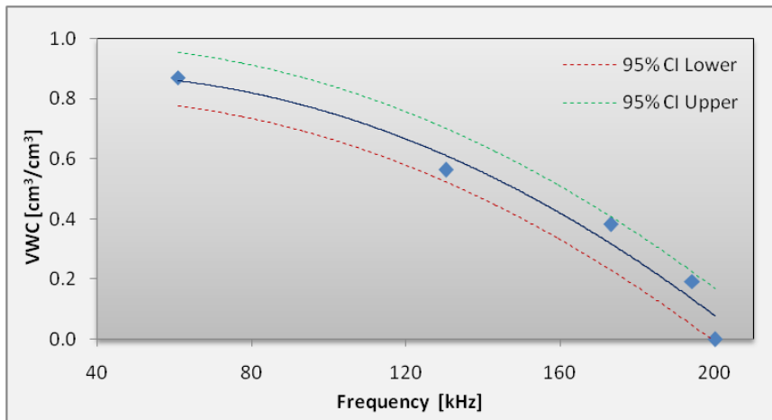
Figure 3. Sensor measurements and calibration curve in mineral wool
