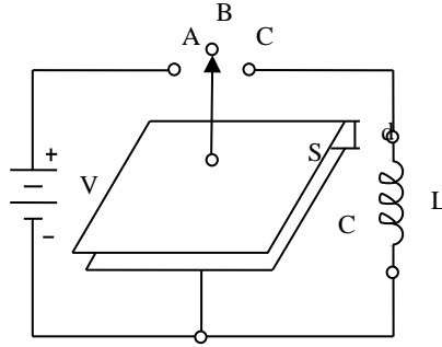
Figure 1. Schematic diagram of a parallel plate capacitor
