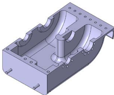
Fig. 4: Parametrically designed reductor housing.
