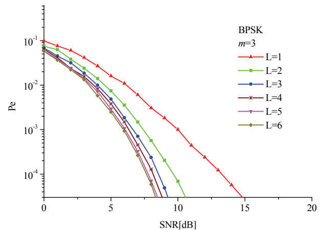
Fig. 8. Bit Error Rate dependence on average SNR for different values of diversity order in Weibull channel
